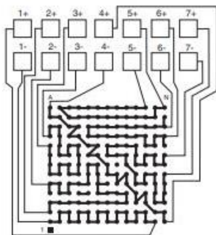
BGA169 AFTER MOUNTING TO TEST BOARD
