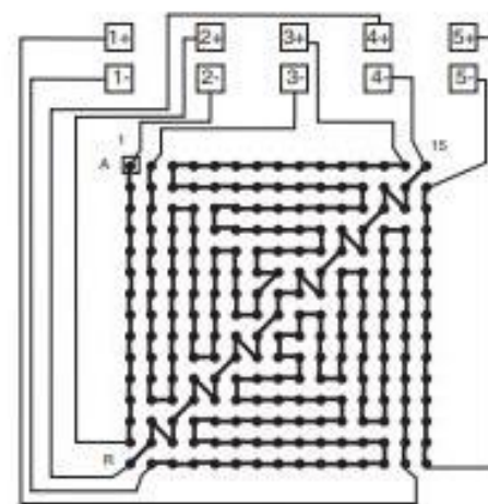
BGA225 AFTER MOUNTING TO TEST BOARD
