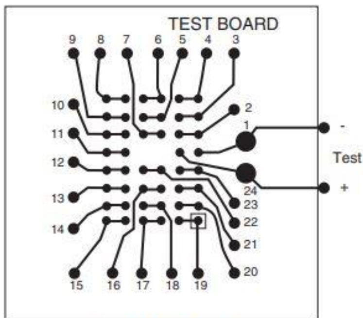
SINGLE PCB TEST COUPON
