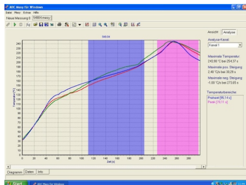
Typical lead free profile 548.04G
