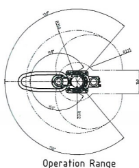
Operation Range
